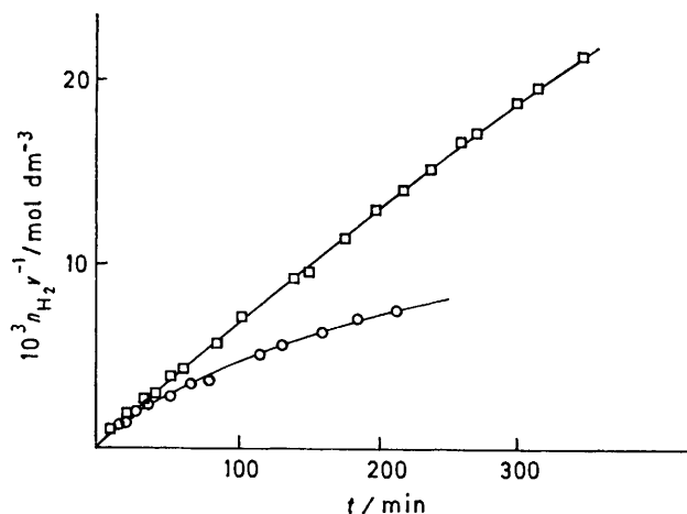
FIGURE 7 \text{H}_2 absorption curves for pyridinecobaloxime(II) recorded in the absence (O) and presence (□) of excess of dimethylglyoxime ( 16 \times 10^{-3} mol \text{dm}^{-3} ). [\text{Co}]_T = 4 \times 10^{-3} mol \text{dm}^{-3} , [\text{py}]_T = 80 \times 10^{-3} mol \text{dm}^{-3} , buffer = 0.05 mol \text{dm}^{-3} borax and 0.08 mol \text{dm}^{-3} \text{HClO}_4 , 20 °C
