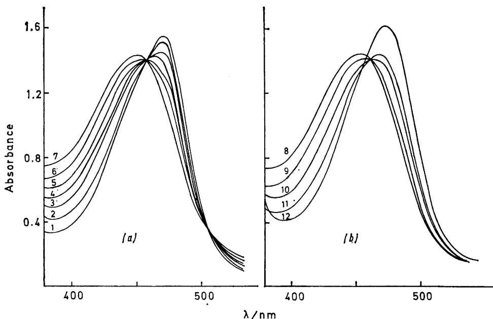
FIGURE 1 Spectra of cobaloxime(II) solutions in MeOH containing increasing amounts of pyridine: (a) [py]_T = 0.0-0.08 mol dm^{-3} ; (b) [py]_T = 0.30-11 mol dm^{-3} ; [Co]_T = 4 \times 10^{-3} mol dm^{-3} ; 20 °C; 0.1 cm cells. [py]_T/mol dm^{-3} = 0 (1), 2 \times 10^{-3} (2), 4 \times 10^{-3} (3), 6 \times 10^{-3} (4), 10 \times 10^{-3} (5), 16 \times 10^{-3} (6), 64 \times 10^{-3} (7), 0.29 (8), 0.58 (9), 1.16 (10), 2.32 (11), and 11.0 (12)
